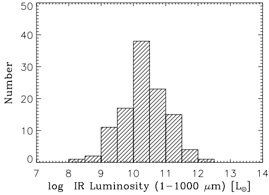
Fig. 8. The IR luminosity distribution, derived from the ISOPHOT Serendipity 170 \mu m and IRAS 100 \mu m and 60 \mu m fluxes. Sources above 10^{12} L_{\odot} are usually called ultraluminous.
