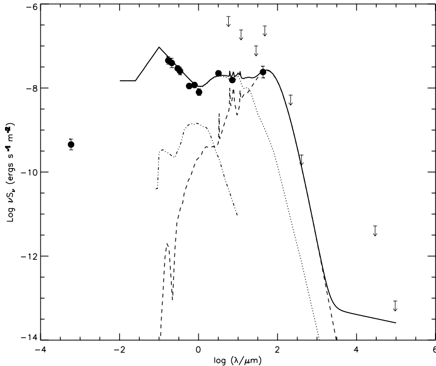
Figure 3. Rest-frame SED of ELAIS J1640+41 from X-rays to radio (data from Table 1). The SED is fitted with a combination of one of the starburst models of Efstathiou et al. (2000b) (dashed line; \tau_V = 50 , t = 26 Myr) and an AGN dusty torus model (dotted line) from Efstathiou & Rowan-Robinson (1995). We assumed a half-opening angle for the torus of 45^\circ and a face-on inclination. The starburst SED is extrapolated in the radio using the far-IR/radio correlation (Helou, Soifer & Rowan-Robinson 1985). For the host galaxy, the SED of a 4-Gyr old stellar population (dotted-dashed line; Fioc & Rocca-Volmerange 1997) has been normalized to K = 17.0 \pm 0.4 mag (see text).
